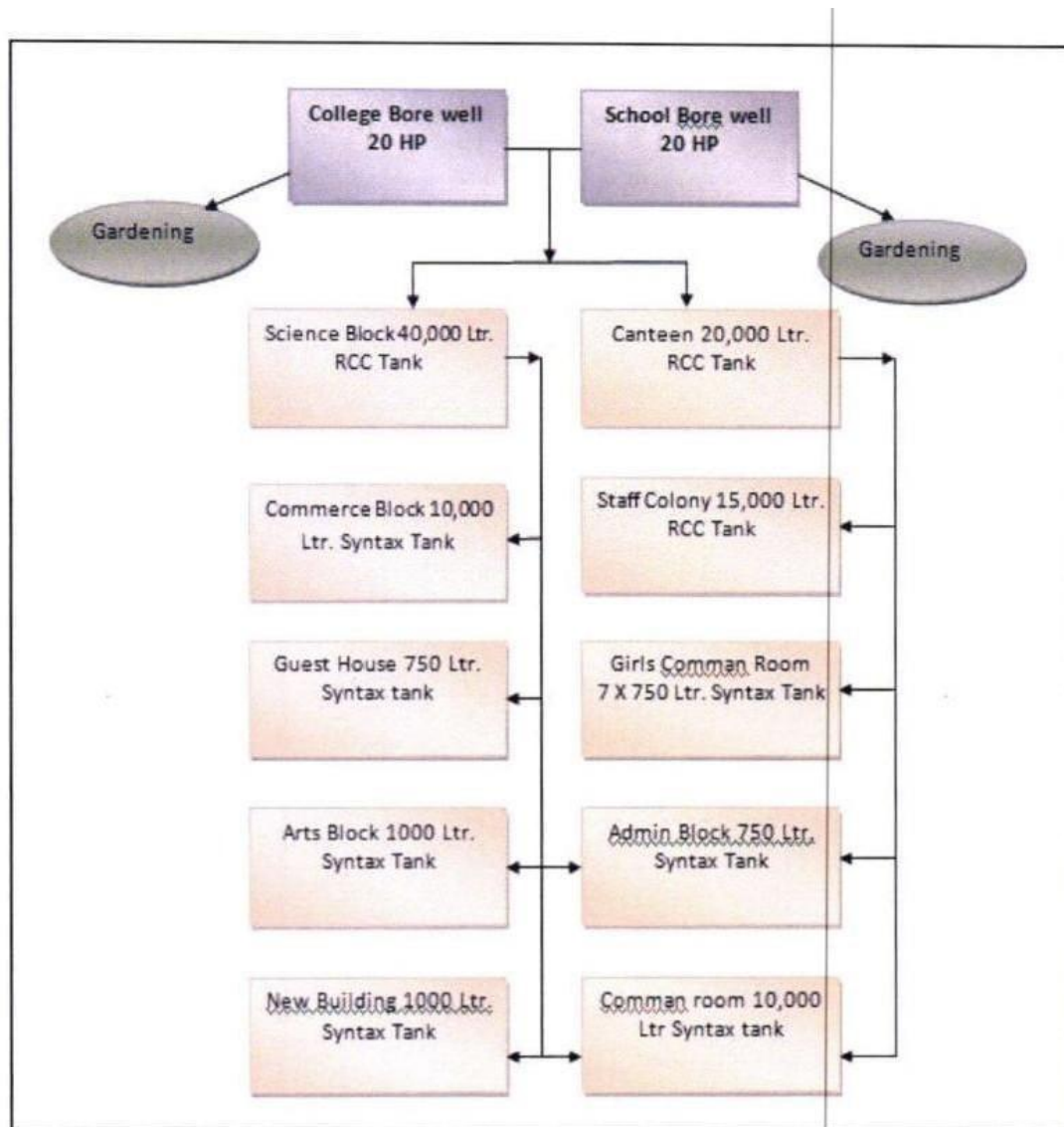
Fig - 2.5 Layout of college Water distribution
